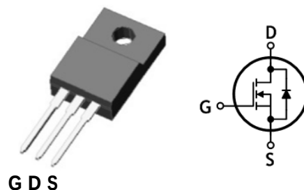
TO-220F-3L
