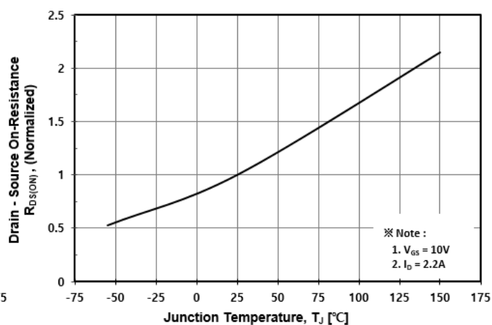
Fig. 8 R_{DS(ON)} - T_J
