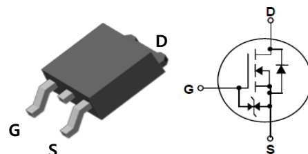
TO-252
