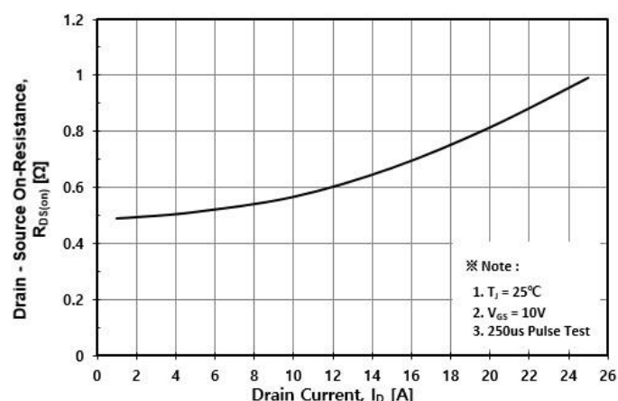
Fig. 3 On-Resistance Variation with Drain Current r_{DS(on)} and Gate Voltage
